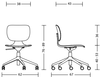
com77 ohne Armlehne without arm supports 8 kg
